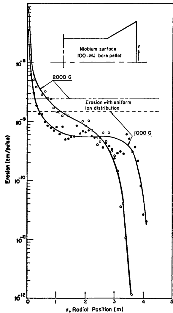
Fig. 13. Sputtering erosion of flat plate energy-sink surface.
