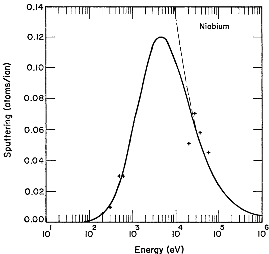
Fig. 4. Sputtering yield of niobium bombarded with \alpha particles.
