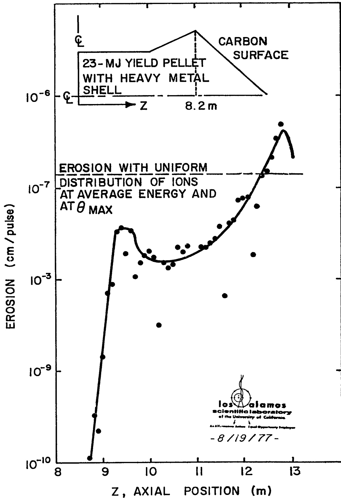
Fig. 14. Erosion of outward-pointing conical energy-sink surface.
