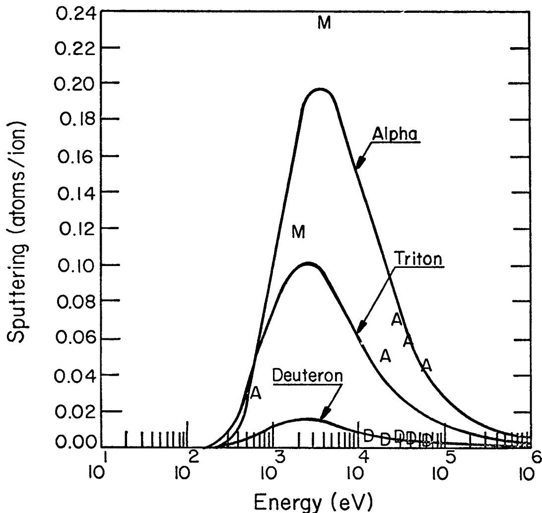
Fig. 7. Sputtering yield of niobium bombarded with \alpha , T^+ and D^+ ions.
