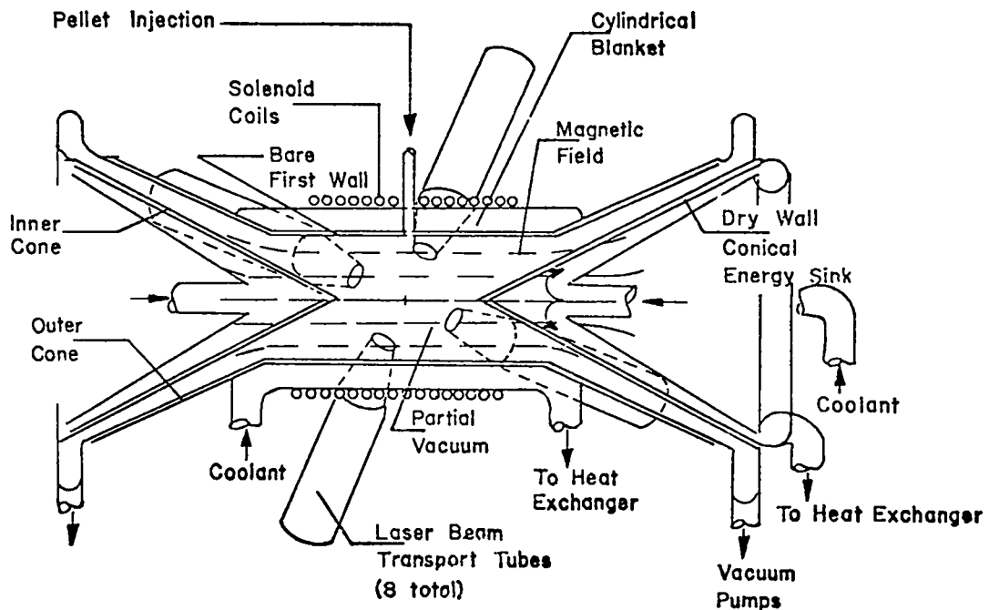
Fig. 1. Cylindrical reactor cavity with magnetically protected wall and conical energy sinks.
