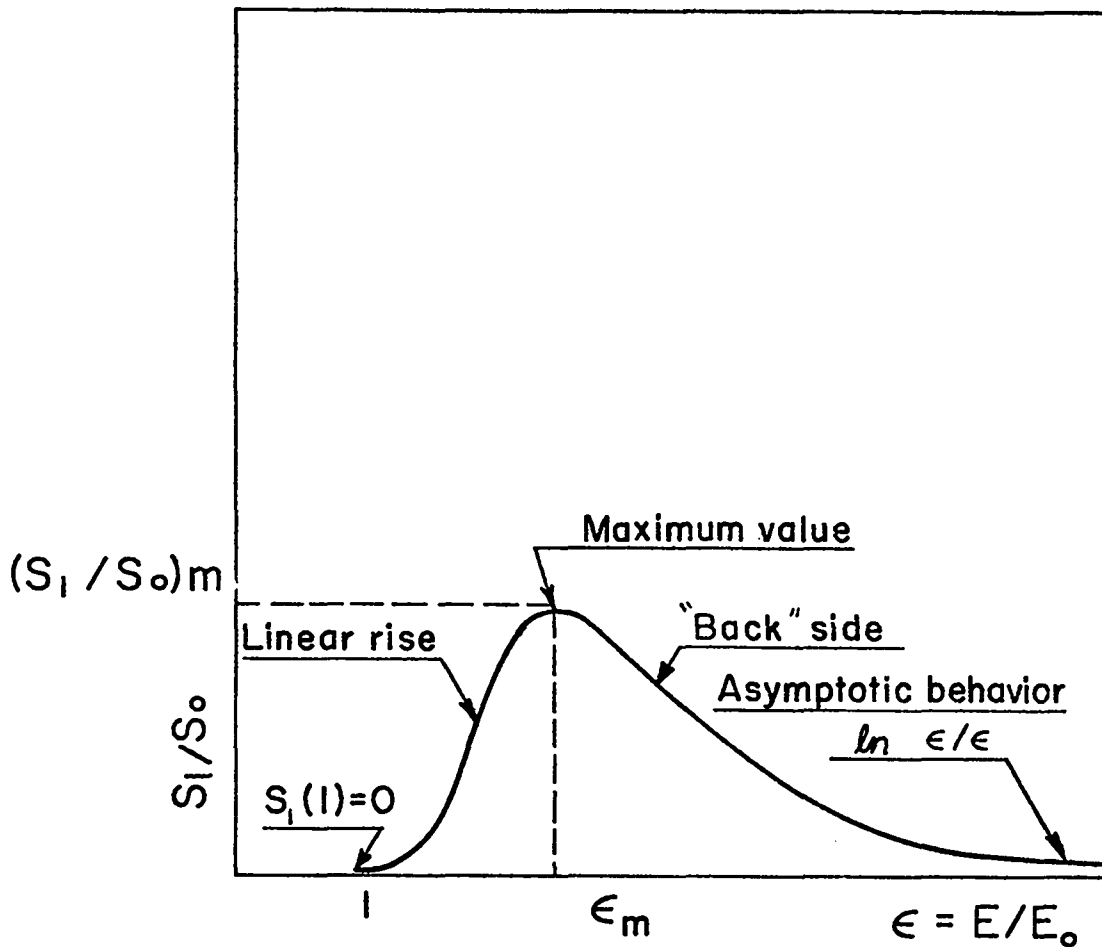
Fig. 2. Energy dependence of sputtering yield--schematic.
