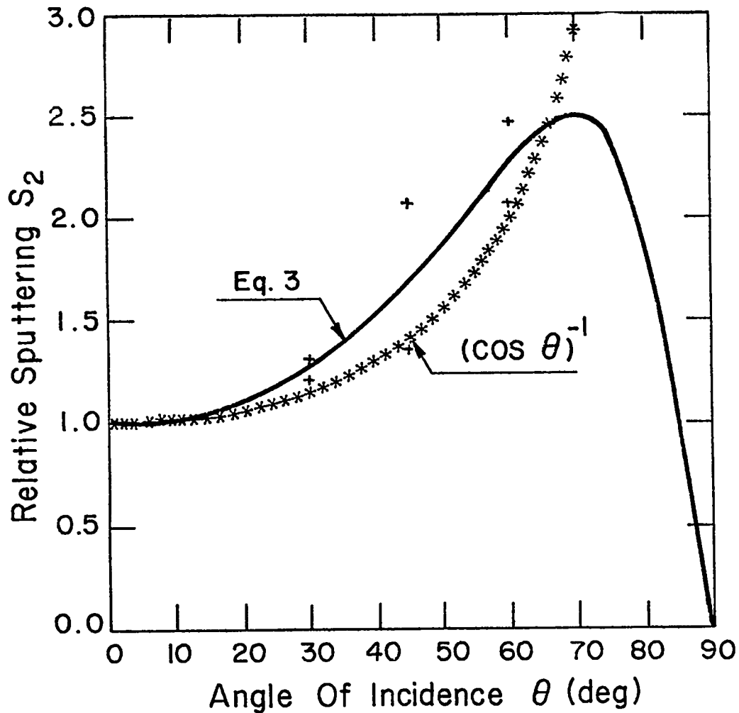
Fig. 3. Dependence of sputtering yield on angle of incidence.
