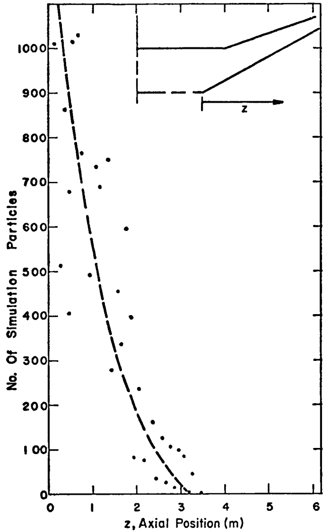
Fig. 10. Ion flux at energy sink surface.
