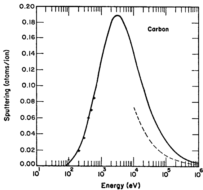
Fig. 6. Sputtering yield of carbon bombarded with \alpha particles.
