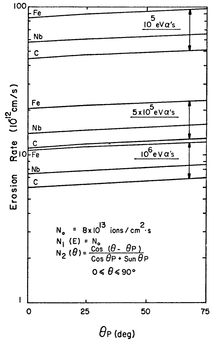
Fig. 9. Angle-of-incidence dependence of erosion rate.
